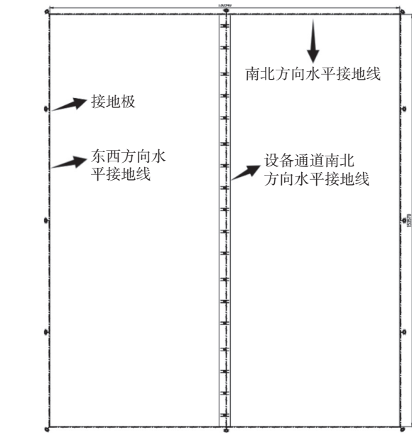
图 10 天津某海上漂浮光伏电站单元方阵防雷接地布置 Fig. 10 Unit array lightning protection grounding layout of a floating photovoltaic power station in Tianjin
