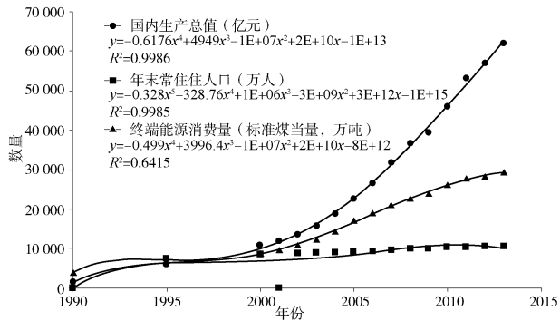
图8 广东省终端能源消费随人口和经济发展的变化 Fig. 8 End-use Energy Consumption Versus Population and Economic Output in Guangdong Province
