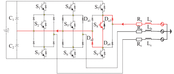
(c) S_8 闭合, I_a > 0 时
